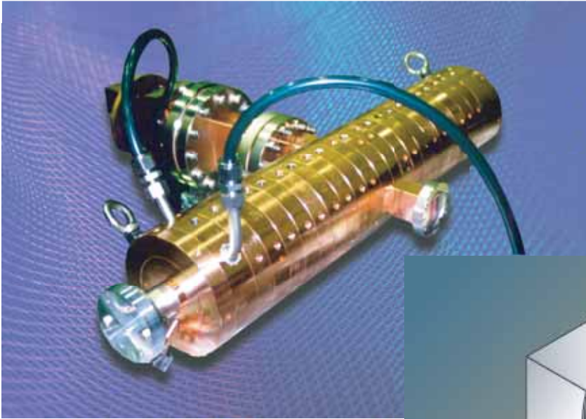
10MeV ON-AXIS COUPLED STANDING WAVE ACCELERATOR
